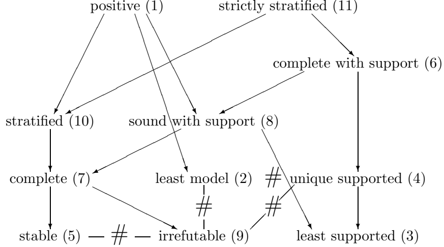
Figure 2: Relations between Solutions 1–11
