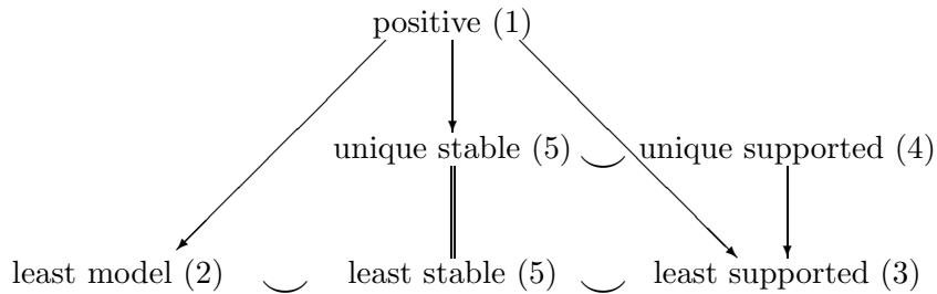
Figure 1: Relations between Solutions 1–5
